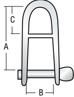
Captive Halyard
