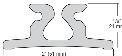
3849 Flanged track
