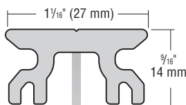
3844 Slug-mount track
