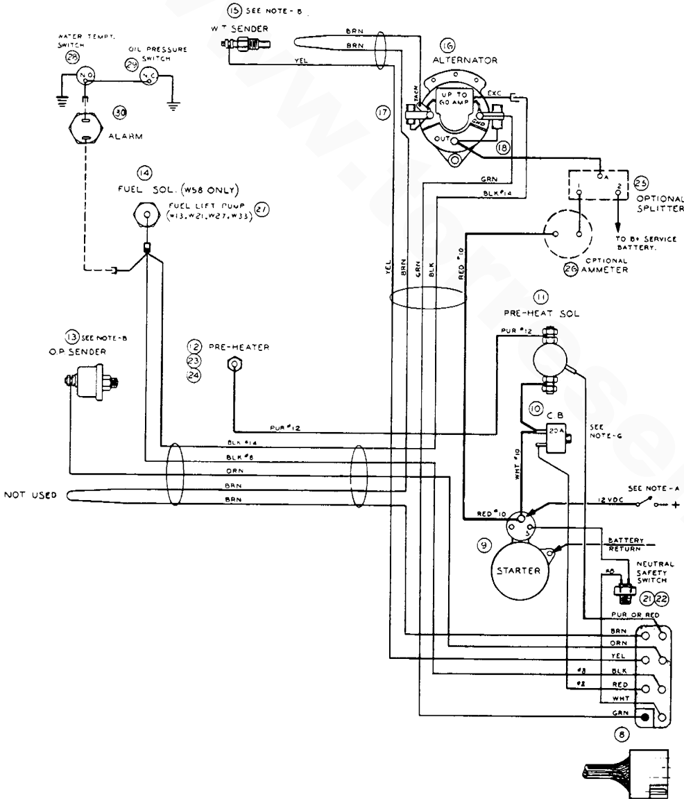
WIRING DIAGRAM
