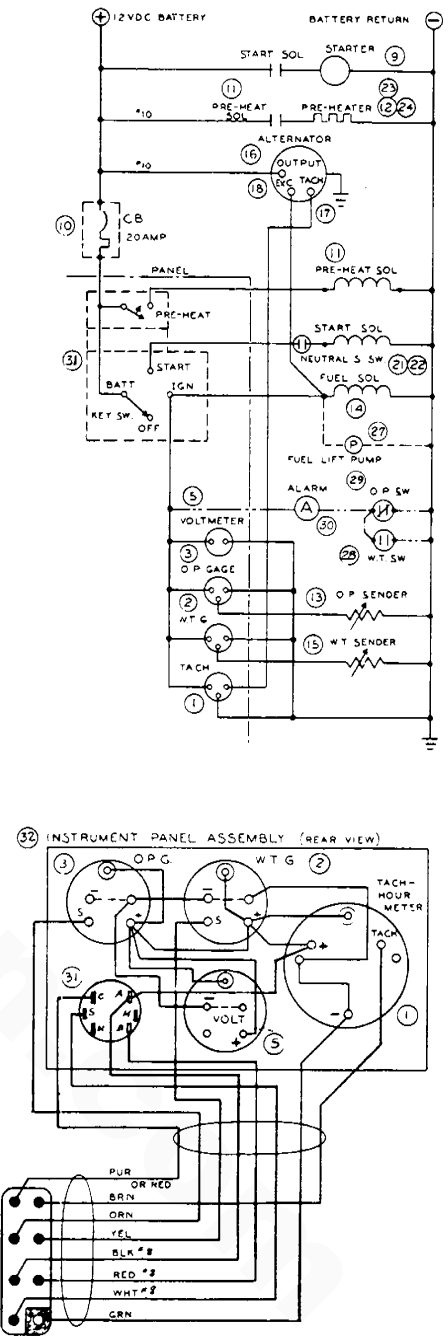
SCHEMATIC DIAGRAM
