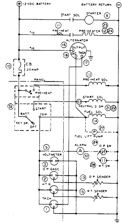
SCHEMATIC DIAGRAM
